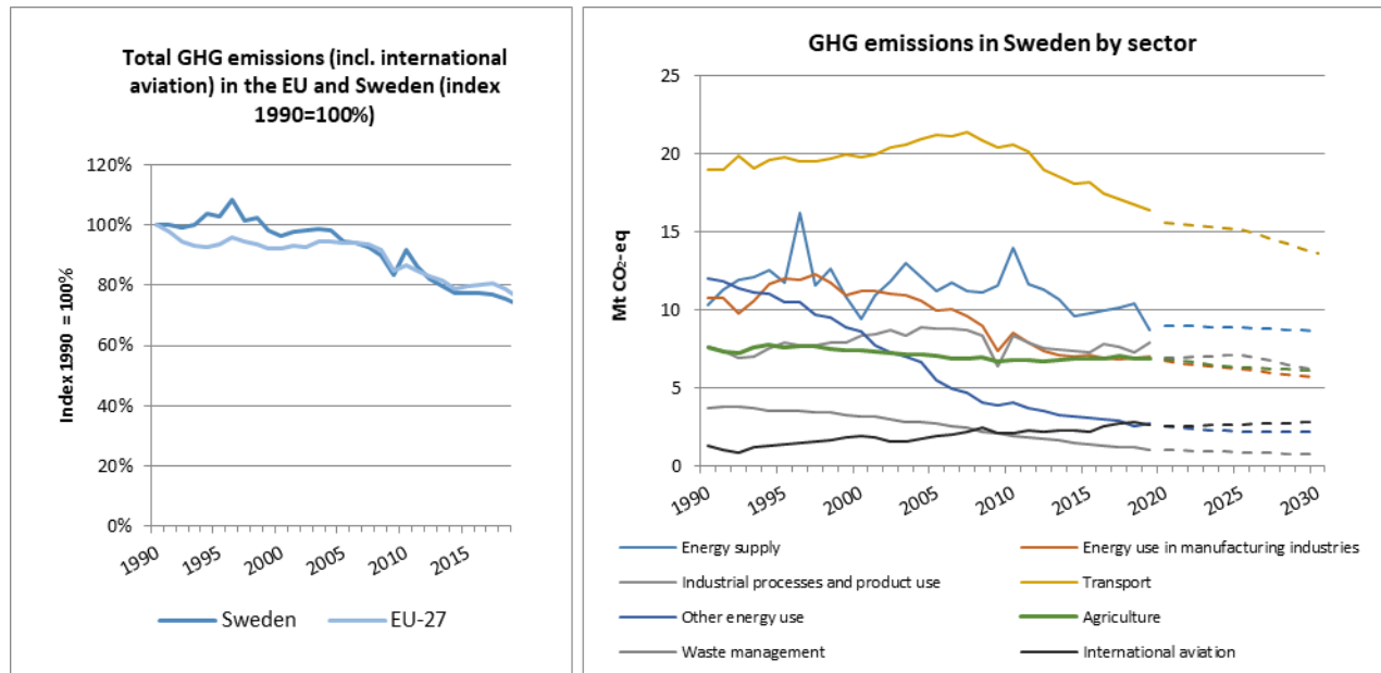
Figure 1: Left hand side: Total greenhouse gas emissions (incl. international aviation) 1990-2020 (index 1990 = 100 %). Right hand side: Greenhouse gas emissions by sector 1 – historical emissions 1990-2019, proxy 2020, projections WEM 2021-2030 (Mt CO 2 -eq).
