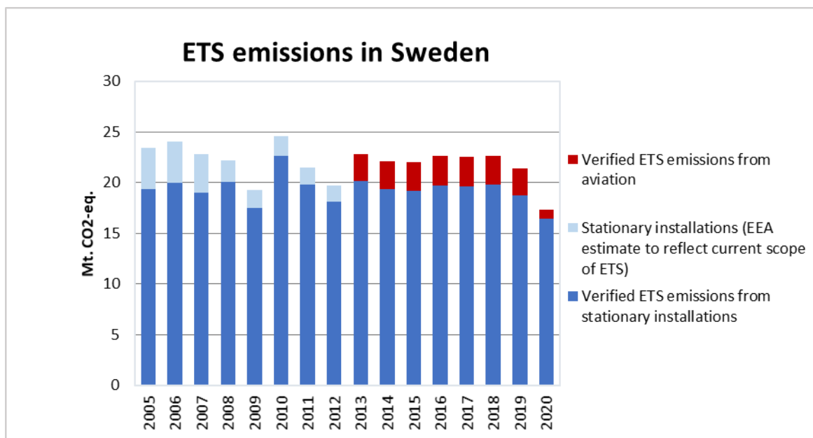
Figure 3: ETS emissions 2005-2020 (Mt CO 2 -eq). 3
