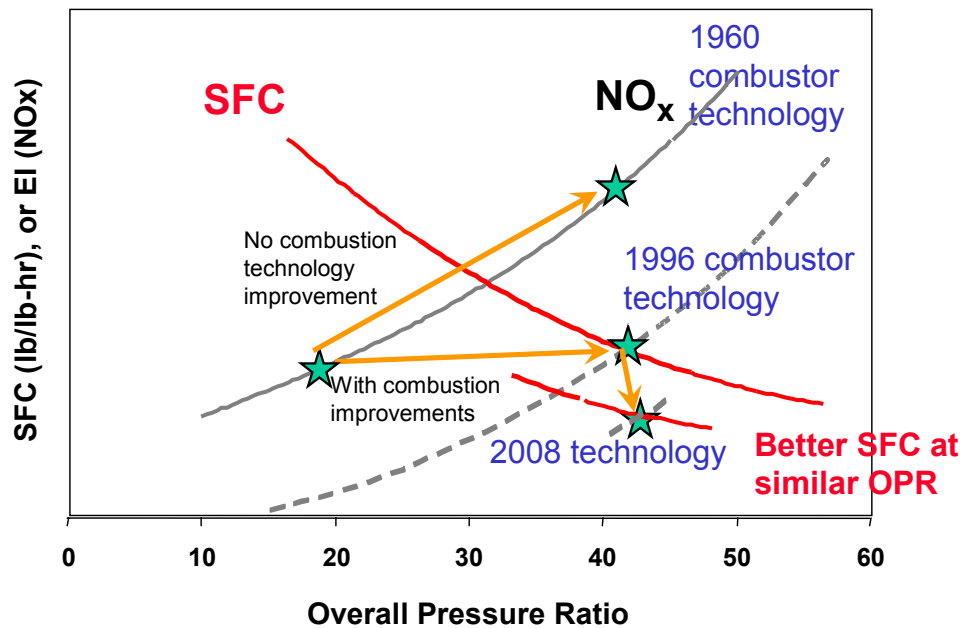
Figure 10 Schematic representation of changes in overall pressure ratio, specific fuel consumption (SFC) and \text{NO}_x emissions index ( \text{EINO}_x ) (courtesy of P. Madden, Rolls-Royce)
